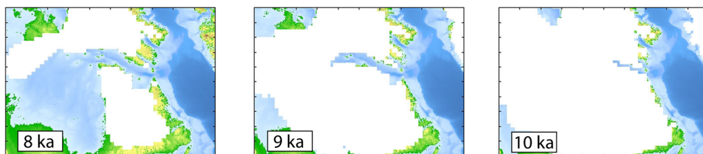
Figure 13. Paleobathymetry and ice cover in the region of Hudson Bay at 8, 9, and 10 ka.
