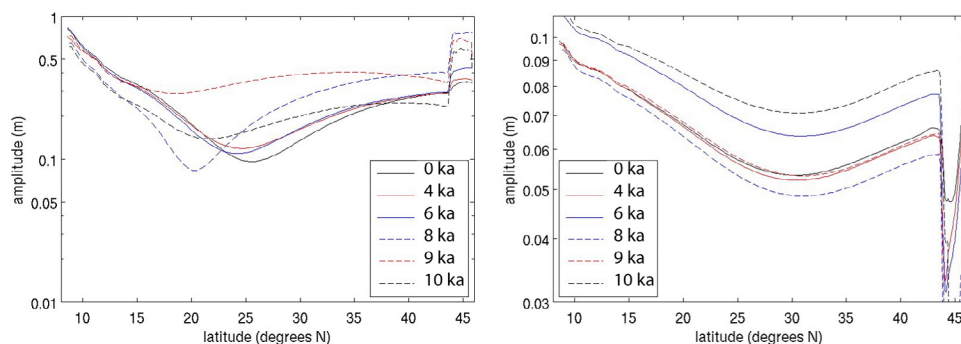
Figure 6. Tidal amplitudes from the global model at 60^{\circ}\text{W} at various points in time. (left) M_2 . (right) K_1 .
